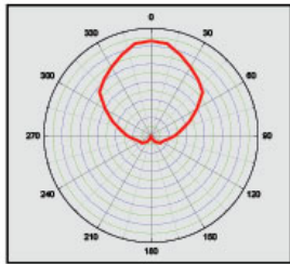
POLAR CURVE:
